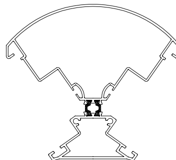
CRS 9530A skypod ACUTE Acute ridge body
